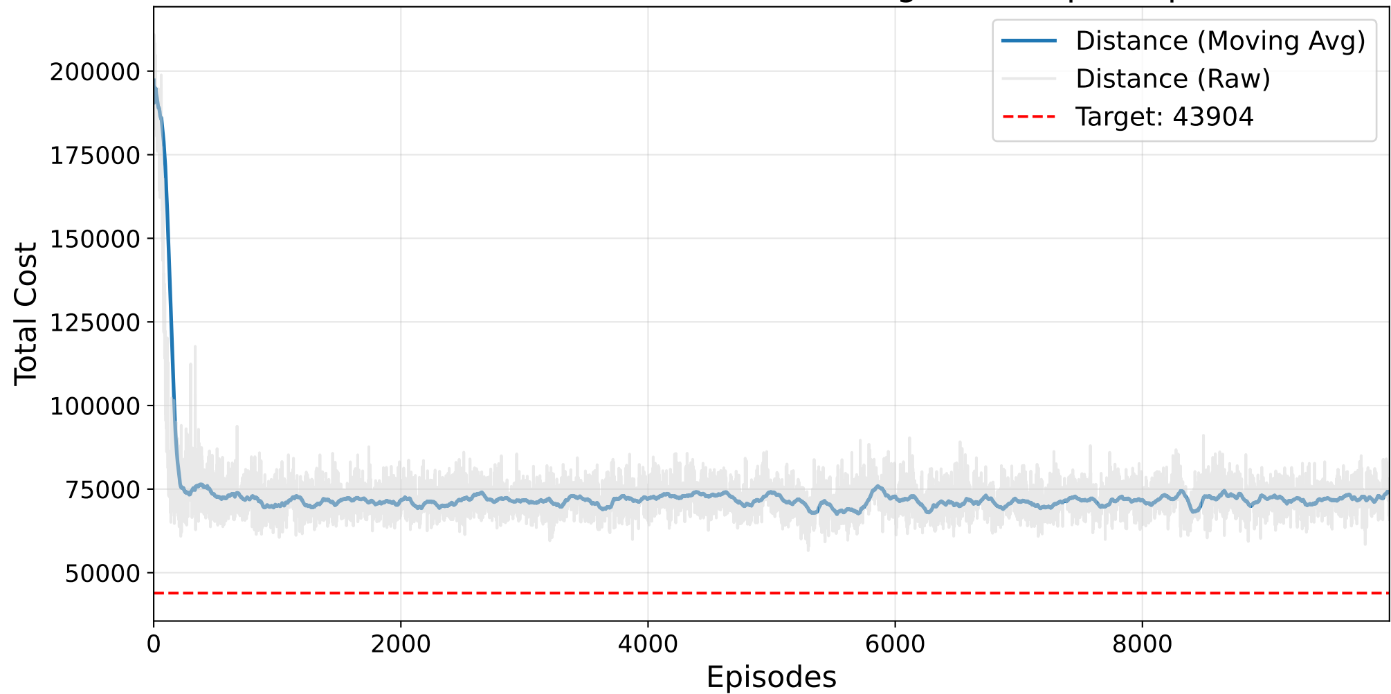
Final Masked AutoRL-SOP Training - kro124p.3.sop
